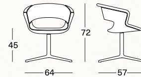
Ⓟ Z020, Ⓜ Z021 Base girevole Swivel base Base pivotante 4-strahliges Fusskreuz, drehbar
